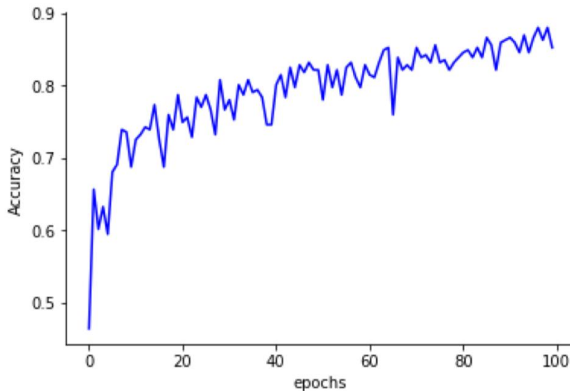
Figure 3. CNN Training Results
