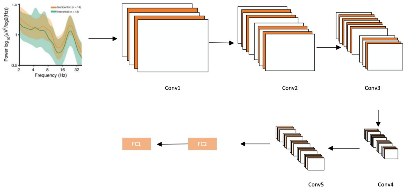
Figure 2. CNN Network Architecture Model
