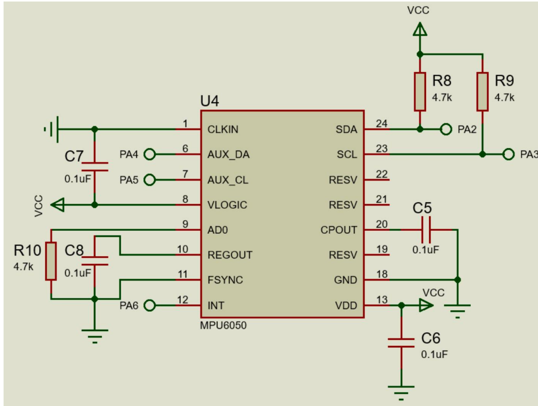
Figure 5. The hardware circuit of the orientation detection sensor MPU6050
