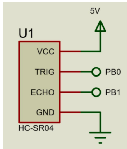
Figure 2. The hardware circuit of the ultrasonic sensor HC-SR04
