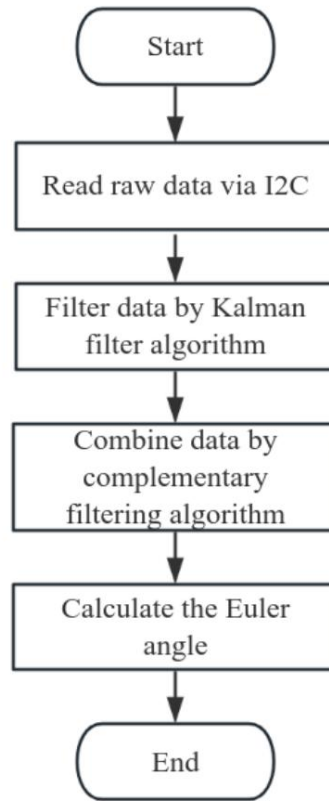
Figure 10. The flow chart of orientation detection program
