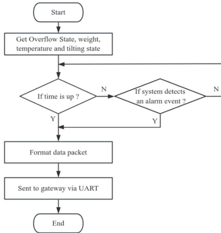
Figure 11. The flow chart of the LoRa communication program
