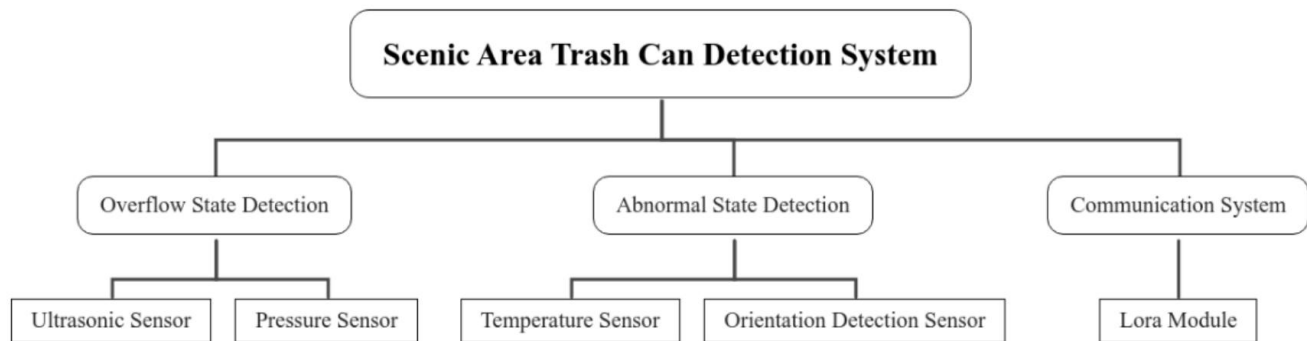
Figure 1. Overall design of scenic area trash can detection system
