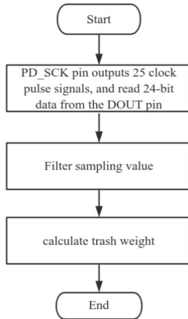
Figure 8. The flow chart of trash weight detection program
