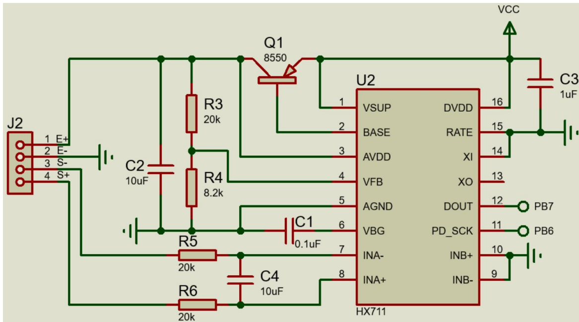
Figure 3. The hardware circuit of the pressure sensor HX711
