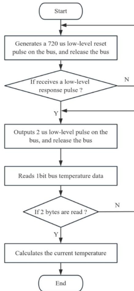
Figure 9. The flow chart of temperature detection program
