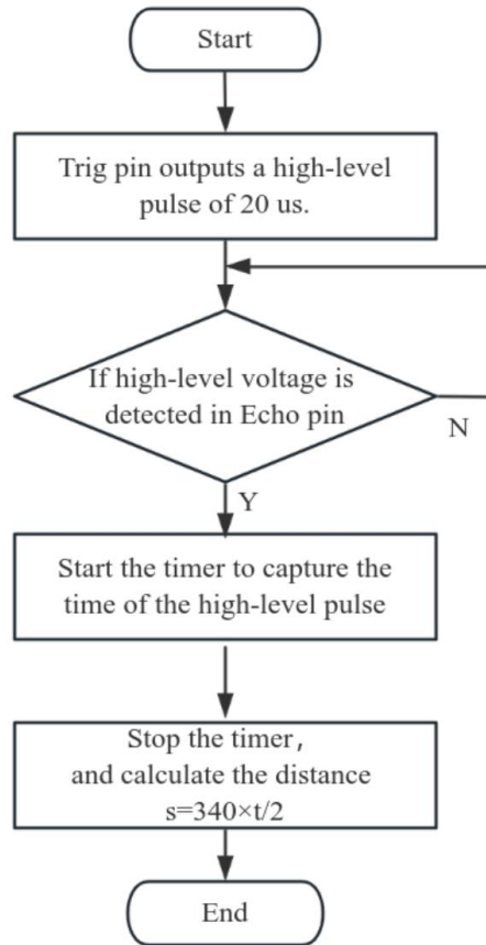
Figure 7. The flow chart of ultrasonic ranging program
