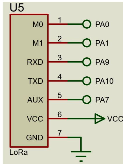
Figure 6. The hardware circuit of LoRa module
