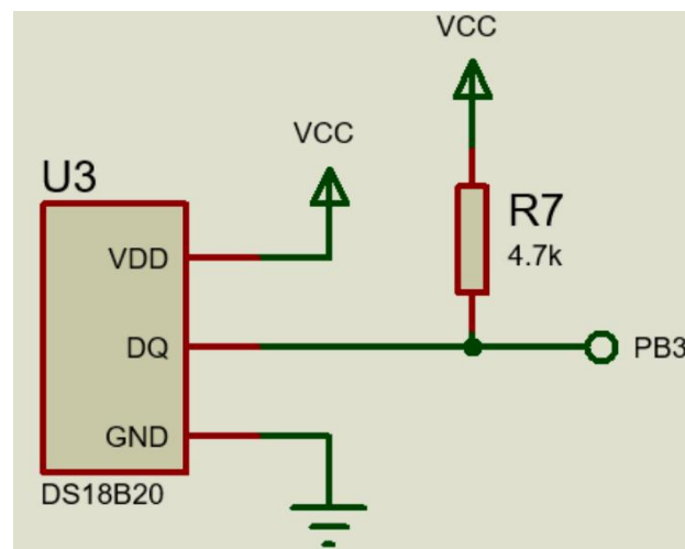
Figure 4. The hardware circuit of the temperature sensor DS18B20
